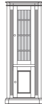
Single Door Glazed Top Corner Unit H 1975mm x W 755mm x D 535mm AFUS139
