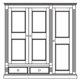
1.8 Ladies Wardrobe H 1950mm x W 1890mm x D 605mm AFWL780
