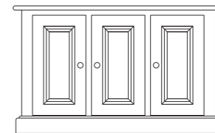
3 Bay Breakfast Bar AFDX533 H 922mm x W 1524mm x D 915mm (Base Unit Dimensions W 1446mm x D 616mm)
