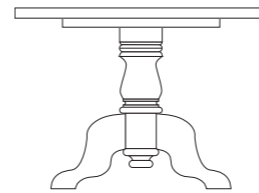
42" Round Farmhouse Table H 762mm x W 1067mm x D 1067mm APTP042
