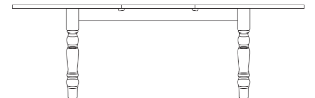
6-3 Extending Great Farmhouse Table H 765mm x W 2384mm x D 915mm APTG634
