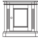
Large Single Door Corner Base H 765mm x W 755mm x D 535mm AFUB130
