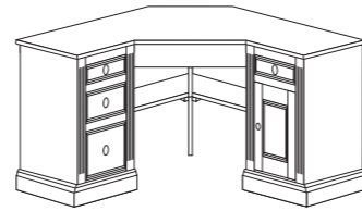
Corner Desk - Combination 5 H 772mm x W 1765mm x D 1250mm AFFC500
