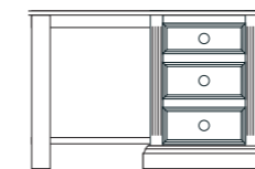
Single Pedestal Dressing Table H 763mm x W 1165mm x D 440mm AFCC100
