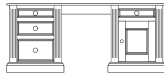
Desk - Combination 5 H 772mm x W 1770mm x D 590mm AFFD500
