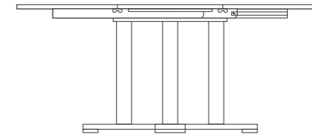
48" Extending Round Pedestal Table H 765mm x W 1829mm x D 1220mm APTP640
