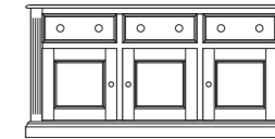
Large 3 Bay Dresser Base H 918mm x W 1860mm x D 590mm AFDR300
