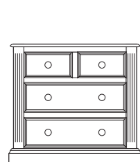
2+2 Chest of Drawers H 916mm x W 1020mm x D 440mm AFCA220
