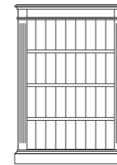
54-38-9 Bookcase AFAB953 H 1372mm x W 960mm x D 290mm
