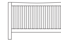
Single Oxford Bed H 1050mm x W 1055mm x D 1995mm APBO120
