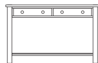
Large Hall Table H 765mm x W 1220mm x D 330mm AKOH414
