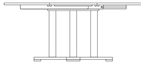
48" Extending Round Pedestal Table H 765mm x W 1829mm x D 1220mm APT640
