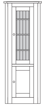
Single Door Glazed Top Corner Unit H 1990mm x W 755mm x D 510mm AKUS139
