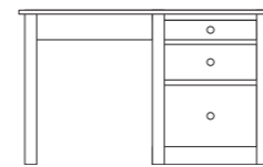
Desk - Single Pedestal 3 Drawers H 782mm x W 1300mm x D 590mm AKFA300
