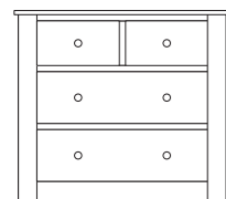
2+2 Chest of Drawers H 926mm x W 1050mm x D 450mm AKCA220
