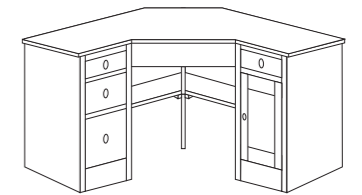
Corner Desk - Combination 5 H 782mm x W 1765mm x D 1250mm AKFC500
