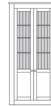
78-38-12 Half Glazed Cabinet AKAH273 H 1982mm x W 970mm x D 345mm
